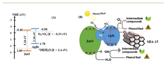
Fig. 7 (A) Schematic of the separation transfer before contact, and (B) possible Z-scheme transfer in the 20%ZnO–Ag@AgBr/SBA-15 photocatalyst.
