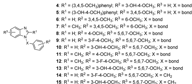
Fig. 2 Structures of 1,2-diarylbenzimidazoles (4 and 5) and 1-arylbenzimidazoles (6–15).
