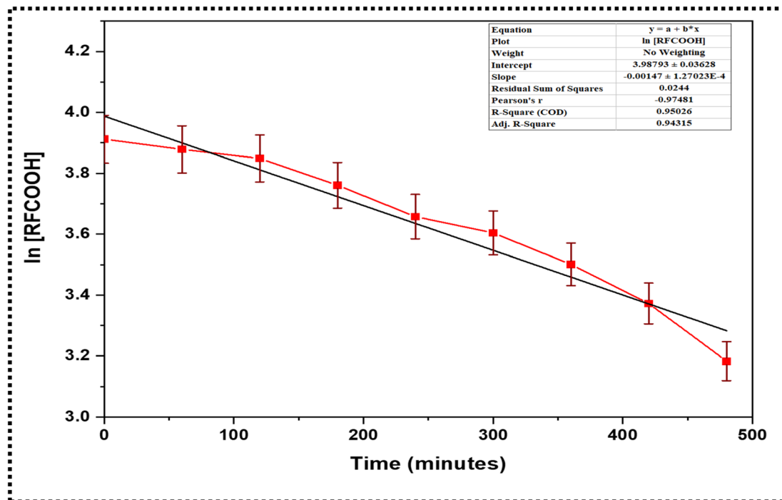
Fig. 5 Kinetic curve of FBAs concentration vs. time.
