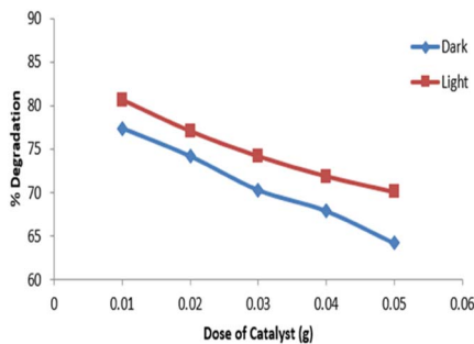
Fig. 11 Effect of catalyst dose on degradation of imidacloprid.
