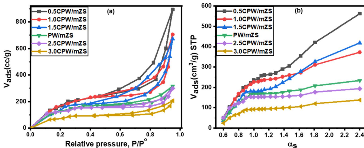
Fig. 2 (a) Adsorption-desorption isotherms of nitrogen at -196\text{ }^{\circ}\text{C} and (b) \alpha_s -plot for PW/mZS and \text{Cs}_x\text{H}_{1-x}\text{PW}_{12}\text{O}_{40}/\text{mZS} samples.
