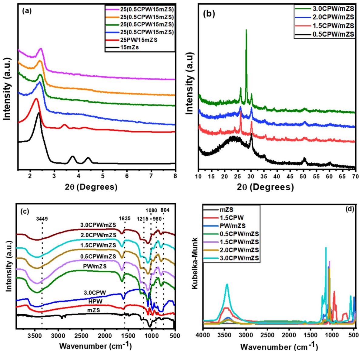
Fig. 1 XRD diffractogram, (a) low-angle, and (b) high-angle patterns, and (c) FT-IR spectra, and (d) FT-IR spectra in coordinate Kubelka–Munk of mZS, HPW, 3.0CPW, PW/mZS, and \text{Cs}_x\text{H}_{3-x}\text{PW}_{12}\text{O}_{40}/\text{mZS} samples.
