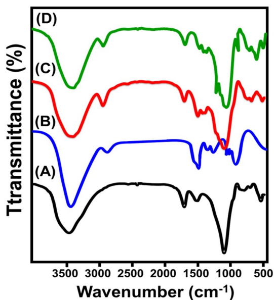
Fig. 3 FT-IR spectra of natural phillipsite (A), cellulose fibers (B), synthetic CF/N.Ph composite (C), and OXPEN encapsulated CF/N.Ph composite (D).
