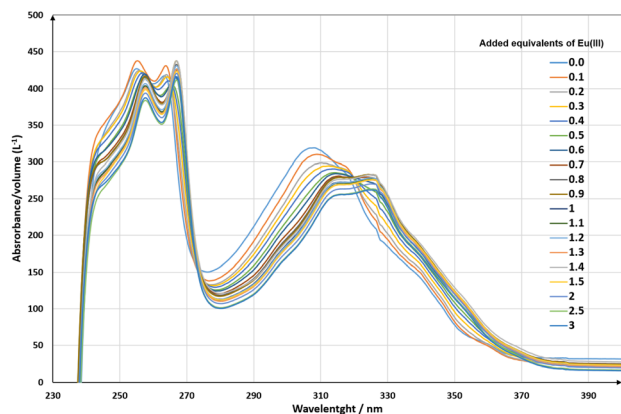
Fig. 13 Spectroscopic titration of DS-BTrzPhen ( 1 ) with \text{Eu}(\text{NO}_3)_3 in neutral water ( I = 0.01 \text{ M Me}_4\text{NNO}_3 ); initial conditions: [\text{DS-BTrzPhen} (\mathbf{1})] = 1 \times 10^{-5} \text{ M} , volume = 2.0 mL; titrant: [\text{Eu}(\text{NO}_3)_3] = 1 \text{ mM} .
