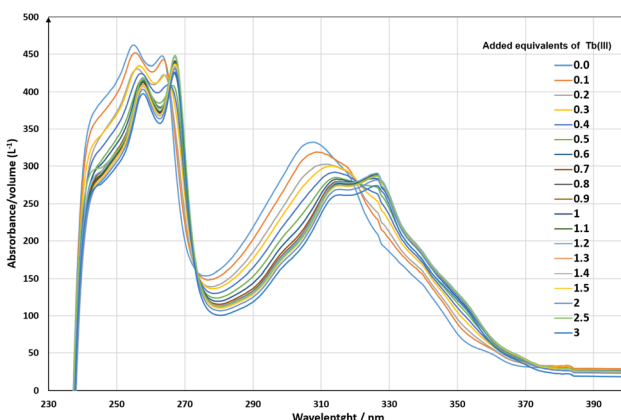
Fig. 14 Spectroscopic titration of DS-BTrzPhen ( 1 ) with \text{Tb}(\text{NO}_3)_3 in neutral water ( I = 0.01 \text{ M Me}_4\text{NNO}_3 ); initial conditions: [\text{DS-BTrzPhen} (\mathbf{1})] = 8 \times 10^{-6} \text{ M} , volume = 2.0 mL; titrant: [\text{Tb}(\text{NO}_3)_3] = 1 \text{ mM} .
