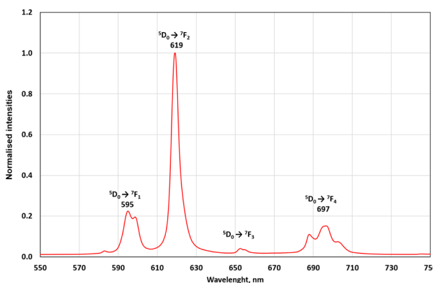
Fig. 15 Fluorescence emission spectrum of DS-BTrzPhen-Eu complex (0.2 mM, molar ration 2 : 1) in water at excitation wavelength of 326 nm.
