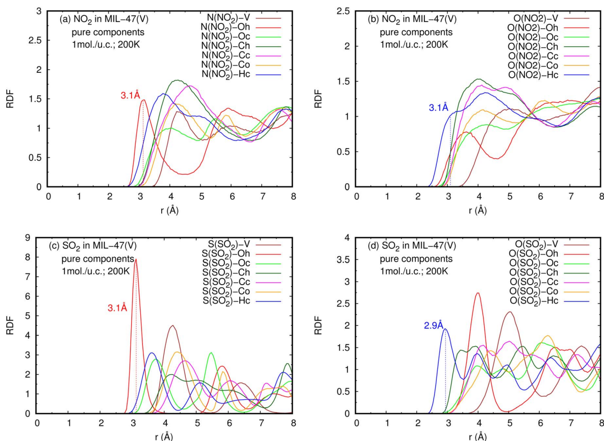
Fig. 7 RDFs of (a), (b) NO 2 –lattice atoms and (c), (d) SO 2 –lattice atoms in pure component, at loading of 1 mol per u.c. and 200 K.
