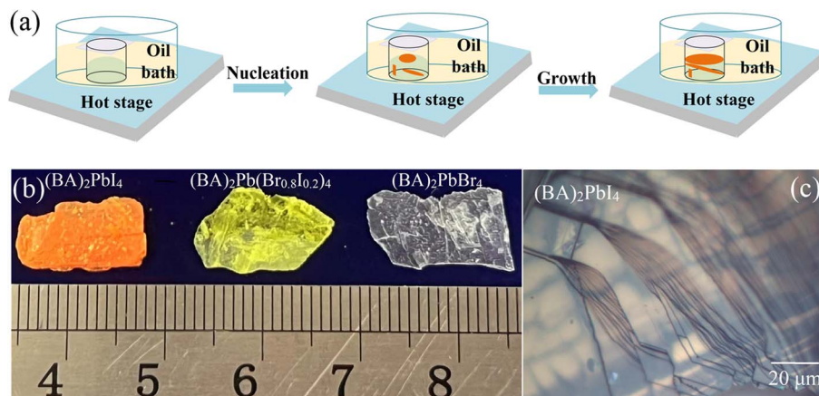
Fig. 1 (a) Schematic of the procedure to grow the mixed halide 2D perovskite (\text{BA})_2\text{Pb}(\text{Br}_x\text{I}_{1-x})_4 single crystals. (b) (\text{BA})_2\text{PbI}_4 , (\text{BA})_2\text{Pb}(\text{Br}_{0.8}\text{I}_{0.2})_4 , and (\text{BA})_2\text{PbBr}_4 single crystals (from left to right). (c) (\text{BA})_2\text{PbI}_4 single crystal.
