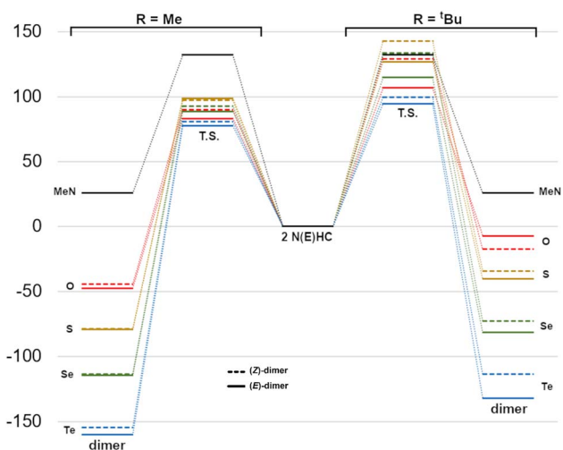
Fig. 7 Reaction Gibbs energy diagram for dimerization ( \text{kJ mol}^{-1} ) of \text{Me}_2\text{im} and the NEHCs (centre) to give methyl- (left) or tert -butyl-substituted dimers (right).
