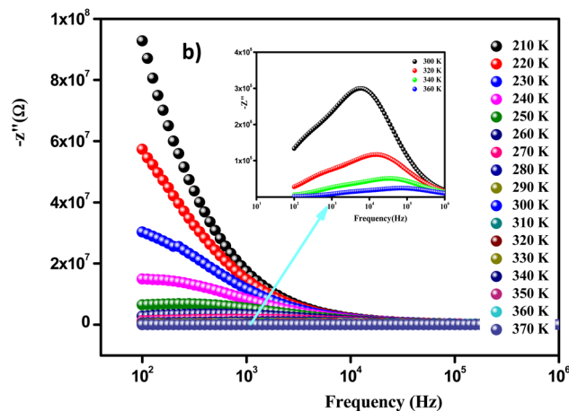
Fig. 9 Frequency evolution of the real part of the impedance plot of \text{Li}_{0.08}\text{Mn}_{0.92}\text{NbO}_4 compound at selected temperatures (a). Frequency evolution of the imaginary part of the impedance plot of \text{Li}_{0.08}\text{Mn}_{0.92}\text{NbO}_4 compound at selected temperatures (b).
