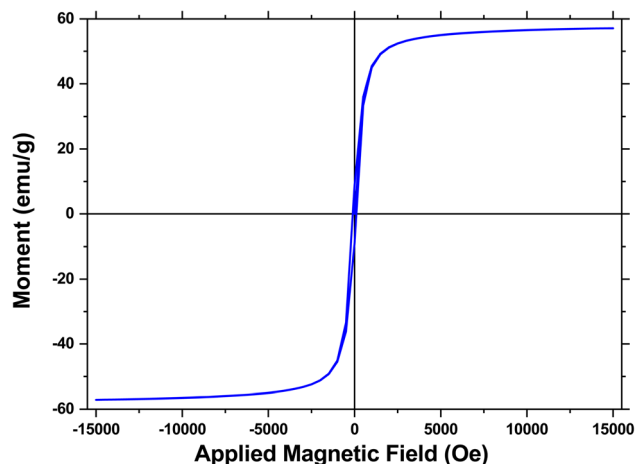
Fig. 8 VSM analysis of [\text{Fe}_3\text{O}_4@Cu^{(III)}(\text{Met})(\text{Pro-H})_2] complex.
