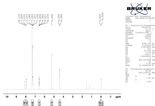
Fig. 3 1 H NMR spectrum of the byproduct.
