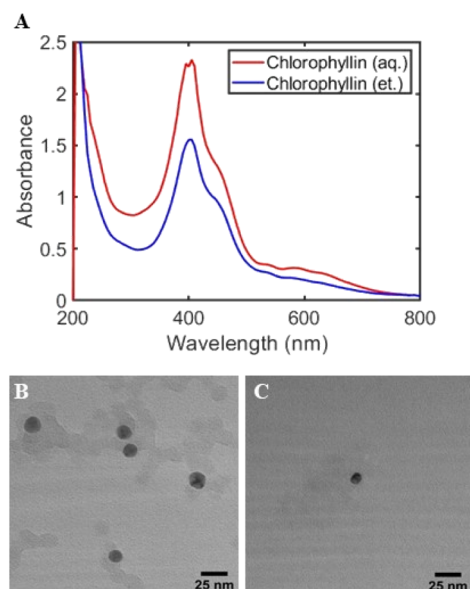
Fig. 6 (A) UV-visible spectra of Ag nanoparticles formed using an aqueous (red curve) and ethanolic (blue curve) chlorophyllin standard. Representative TEM images of Ag nanoparticles synthesized with an (B) ethanolic and (C) aqueous kudzu chlorophyllin standard.
