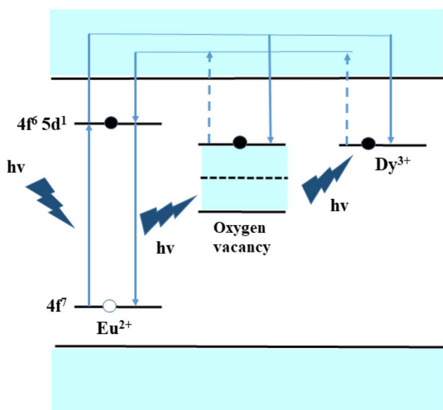
Fig. 6 The representation of the possible excitation-emission process between Dy 3+ and Eu 2+ ions through an energy level diagram.
