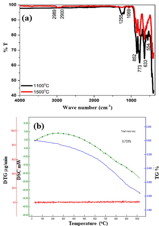
Fig. 4 (a) A comparative FTIR analysis of \text{SrAl}_2\text{O}_4:\text{Eu}^{2+}/\text{Dy}^{3+} annealed at two different temperatures. In the inset of (a), the magnified plot in the range of 400\text{--}1000\text{ cm}^{-1} is shown. (b) Thermogravimetric analysis (TGA), derivative thermal gravimetric (DTG), and difference scanning calorimetric analysis of the thermally optimized sample (annealed at 1500 °C) in the range of 30\text{--}1000\text{ °C} .
