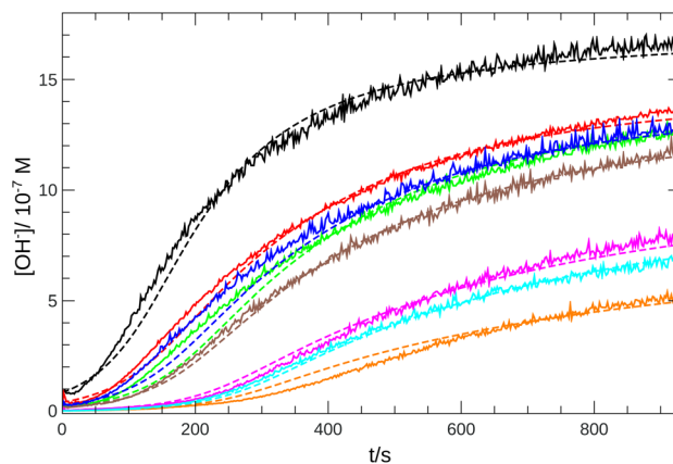
Fig. 2 Time evolution of the [OH^-] for imine "A" with 1 mM reactant concentration. Initial pH decreases from black to orange: 6.92 (black), 6.59 (red), 6.42 (blue), 6.30 (green), 6.22 (brown), 5.64 (magenta), 5.43 (cyan), 5.35 (orange). Experimental measurements are shown with solid lines and the simulated curves with dashed lines.
