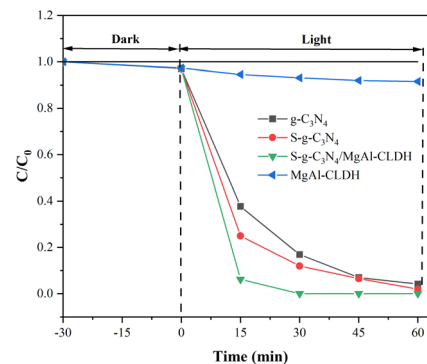
Fig. 10 Photocatalytic degradation of RhB by g-C 3 N 4 , S-g-C 3 N 4 , MgAl-CLDH and S-g-C 3 N 4 /MgAl-CLDH.
