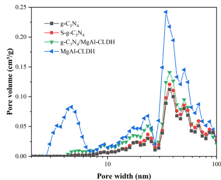
Fig. 7 Pore size distribution of g\text{-C}_3\text{N}_4 , S\text{-}g\text{-C}_3\text{N}_4 , MgAl\text{-CLDH} and S\text{-}g\text{-C}_3\text{N}_4/MgAl\text{-CLDH} .
