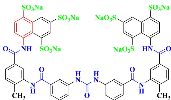
Suramin
