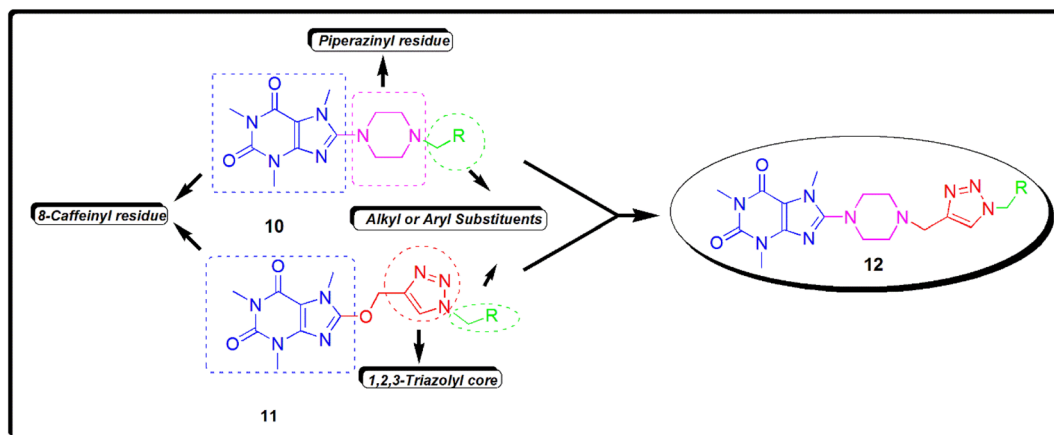
Fig. 4 The structure of new 8-piperazinyl caffeinyl-triazolylmethyl hybrid conjugates 12 and comparing its structure with previously synthesized compounds 10 and 11 .
