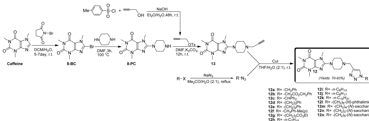
Scheme 1 General synthetic pathway for preparing novel 8-piperazinyl caffeinyl-triazolylmethyl hybrid conjugates 12 .
