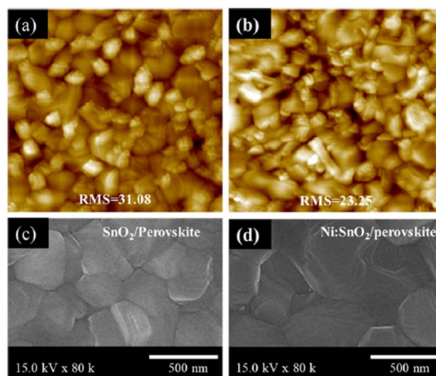
Fig. 9 Material images of (a) AFM for bare \text{SnO}_2 , (b) AFM for Ni-doped \text{SnO}_2 , (c) SEM for bare \text{SnO}_2 , and (d) SEM for Ni-doped \text{SnO}_2 . Reproduced with permission from ref. 57. Copyright 2022 American Chemical Society.
