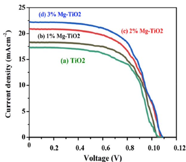
Fig. 8 J–V characteristics of PSC based on (a) bare \text{TiO}_2 , (b) 1% Mg-doped \text{TiO}_2 , (c) 2% Mg-doped \text{TiO}_2 , and (d) 3% Mg-doped \text{TiO}_2 . Reproduced with permission from ref. 49. Copyright 2021 Elsevier.
