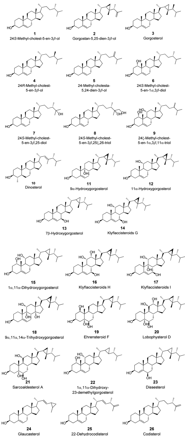
Fig. 2 Tested steroid derivatives 1–26.
