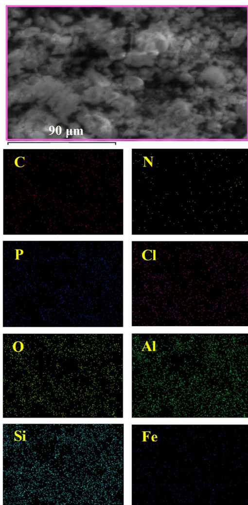
Fig. 4 Energy dispersive X-ray (EDX) mapping analysis of [(\text{APTDP})(\text{FeCl}_4)_2@ \text{HNT}] .
