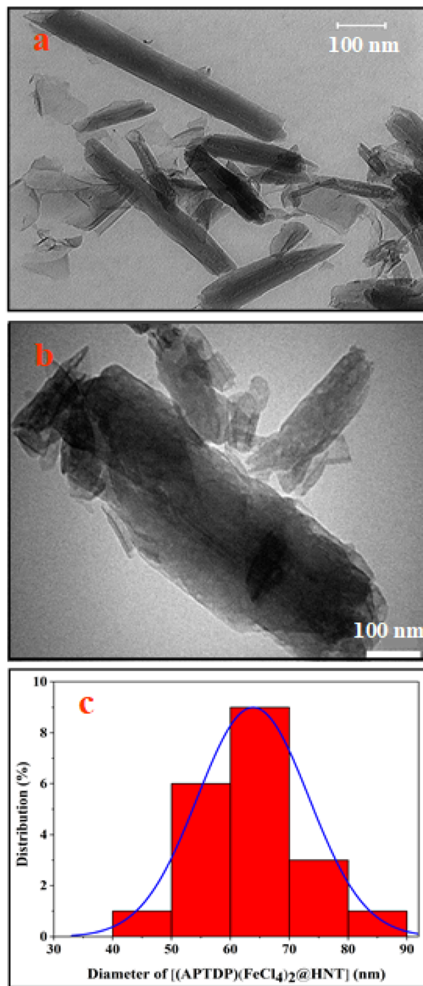
Fig. 5 TEM image of: (a) \text{HNT} , (b) [(\text{APTDP})(\text{FeCl}_4)_2@ \text{HNT}] and (c) particle size distribution for [(\text{APTDP})(\text{FeCl}_4)_2@ \text{HNT}] .
