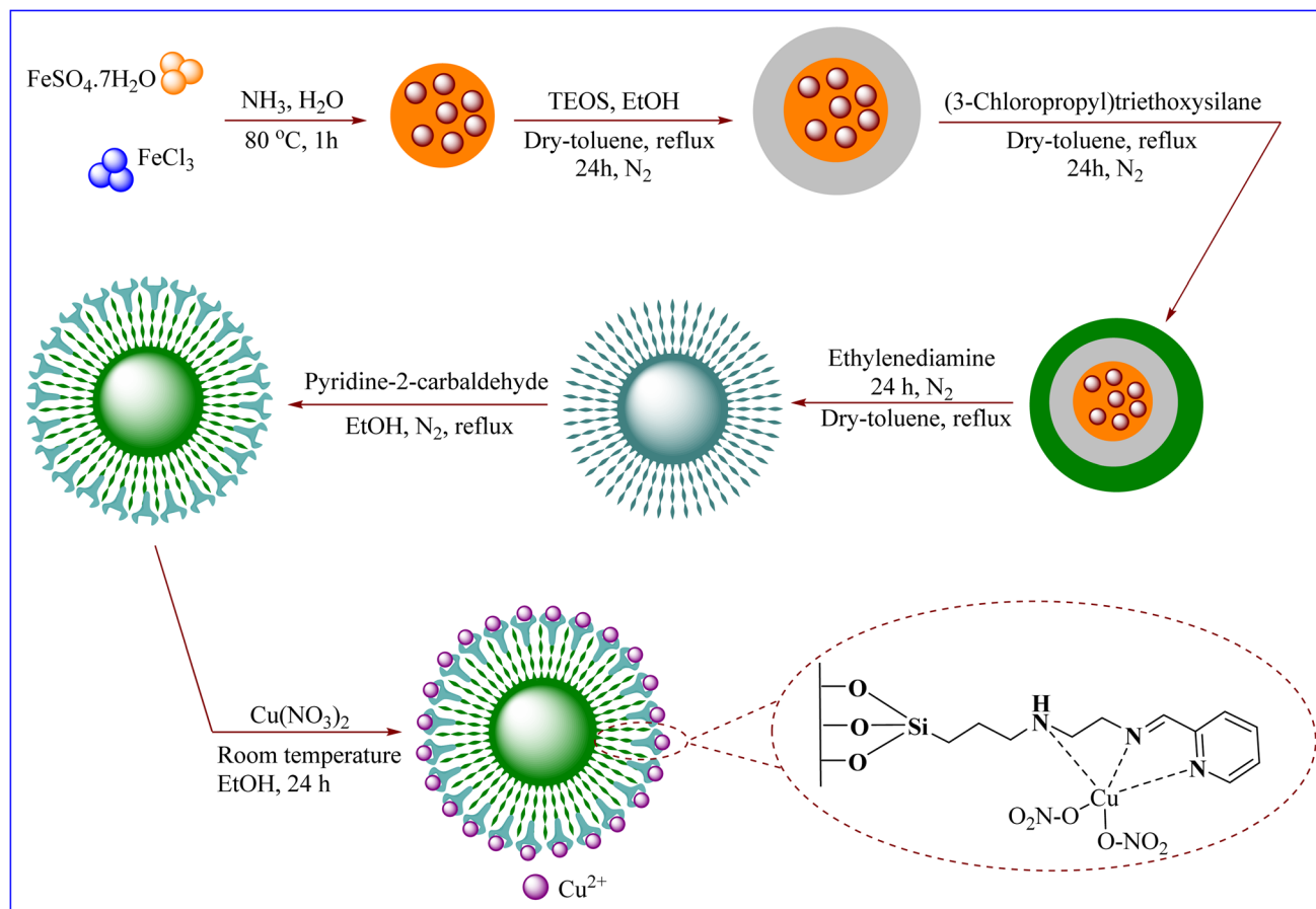
Scheme 2 Synthetic route of magnetic \text{Cu}(\text{II}) -Schiff-base- (\text{CH}_2)_3@\text{SiO}_2@\text{Fe}_3\text{O}_4
