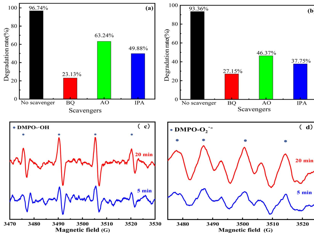
Fig. 12 \text{SnO}_2\text{-AgBr} (1 : 1) composite trapping experiments for (a) MO and (b) MG; EPR spectra of the \text{SnO}_2\text{-AgBr} (1 : 1) composite: (c) \text{DMPO}\cdot\text{OH} , (d) \text{DMPO}\cdot\text{O}_2^- .
