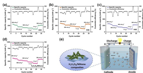
Fig. 4 The rate capability and coulombic efficiency of (a) H24, (b) H36, (c) H48 and (d) H_2V_3O_8/MXene composites at current densities of 200, 500, 800, 1000, 2000 and 200 mA\ g^{-1} . (e) A schematic of the assembly structure of the H_2V_3O_8/MXene ARZBs.
