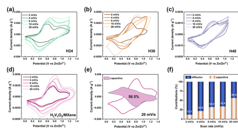
Fig. 3 The CV curves of (a) H24, (b) H36, (c) H48, and (d) the \text{H}_2\text{V}_3\text{O}_8/\text{MXene} composites, respectively. (e) The capacitive contribution of \text{H}_2\text{V}_3\text{O}_8/\text{MXene} , and (f) the capacitive contributions at different scan rates.
