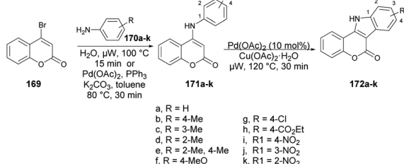
Scheme 61 Synthesis of azacoumestans 172a–k .
