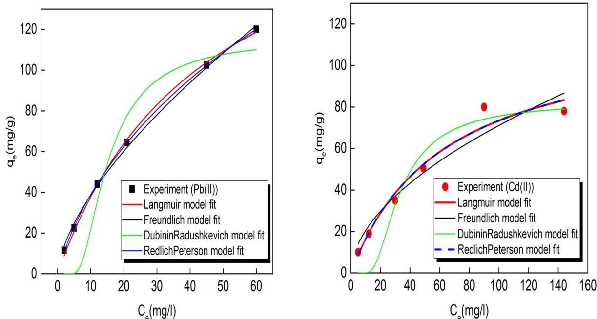
Fig. 7 Adsorption isotherms of Pb(II) and Cd(II) ions (agitation speed: 160 rpm, initial metals concentrations: 25–300 mg L -1 , dose: 2 g L -1 , pH 5.5 and 7 for Pb and Cd(II)).
