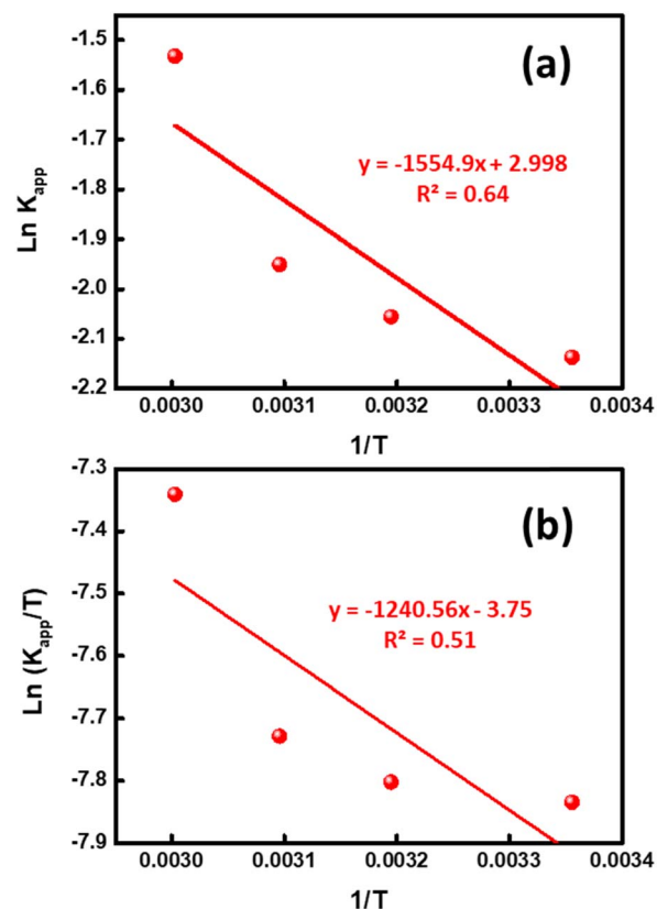
Fig. 8 (a) The plots of \ln K_{app} vs. 1/T and (b) \ln(K_{app}/T) vs. 1/T for the MB degradation using the UiO-66@MoS 2 QDs photocatalyst.
