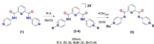
Scheme 1 The synthesis of proligands (2–4) and ligand (5) from (1).
