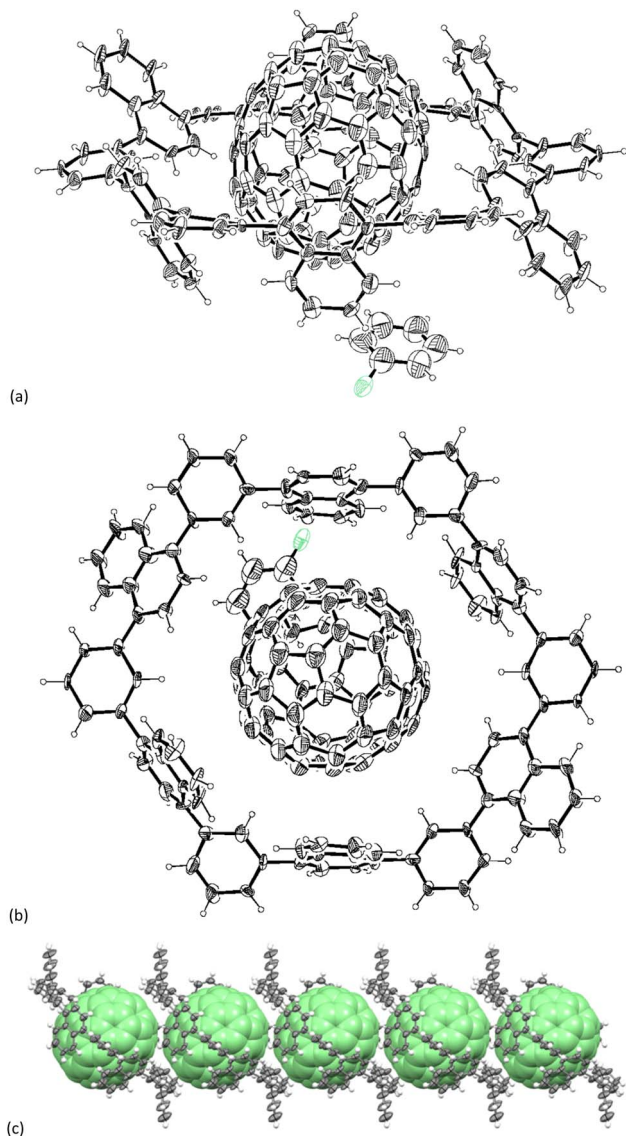
Fig. 4 X-ray structure of the \text{N6-C}_{70} 1:1 complex, ORTEP drawing from (a) the side view and (b) top view with thermal ellipsoids scaled at 25% probability. Disordered molecules are omitted for clarity. (c) A columnar array of \text{N6-C}_{70} along the a -axis. For clarity, \text{C}_{70} is shown as a space-filling model.
