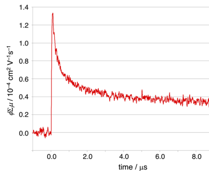
Fig. 5 FP-TRMC profile of the single-crystals ( \text{C}_{60}@\text{N6-PhCl} ) recorded at an excitation wavelength of 355 nm with a photon density of 9.1 \times 10^{15} photons per \text{cm}^{-2} .
