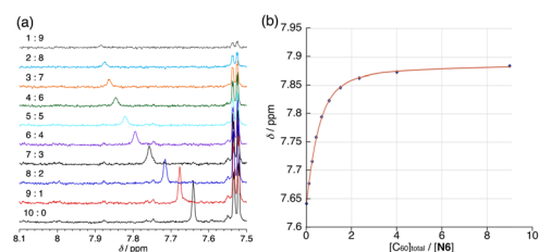
Fig. 2 (a) The chemical shift changes of inside proton resonance observed in ^1\text{H} NMR titration of N6 with C_{60} in toluene- d_8 . ( [N6] : [C_{60}] = 10 : 0 to 1 : 9 , the total concentration was 0.4 mM, 600 MHz, 298 K) (b) curve-fitting obtained by using the 2:1 binding model.
