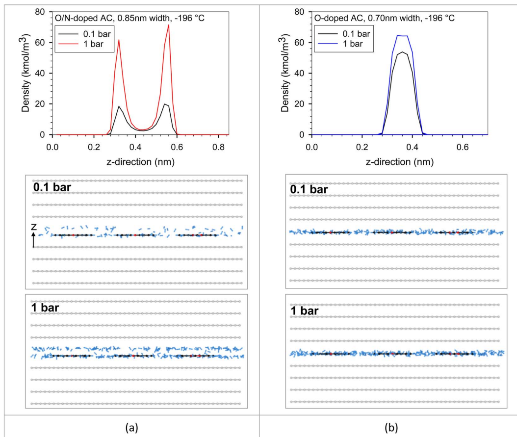
Fig. 14 Local density distributions in z -direction and snapshots of H 2 adsorption in (a) O/N-doped AC model (0.85 nm width) and (b) O-doped AC model (0.70 nm width) at -196^{\circ}\text{C} .
