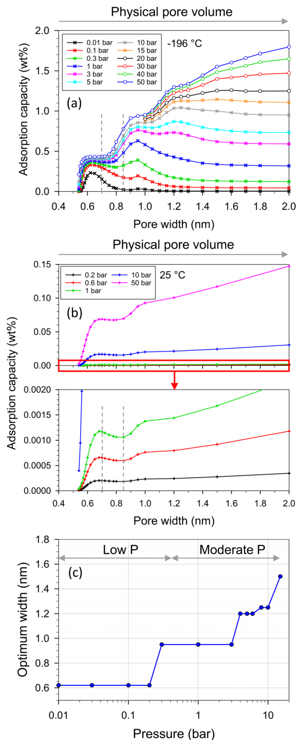
Fig. 12 \text{H}_2 adsorption capacity versus pore width and pore volume at (a) -196 and (b) 25 ^{\circ}\text{C} , (c) optimum width versus pressure at -196 ^{\circ}\text{C} obtained with GCMC.
