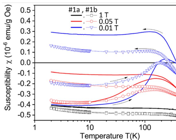
Fig. 11 Zero-field-cooled and field-cooled curves of the CVD samples (#1a: samples after the laser-cut and #1b: after laser-polishing of the laser-cut surface) as a function of temperature between 2 and 380 K at applied fields of 0.01, 0.05, and 1 T. 145
