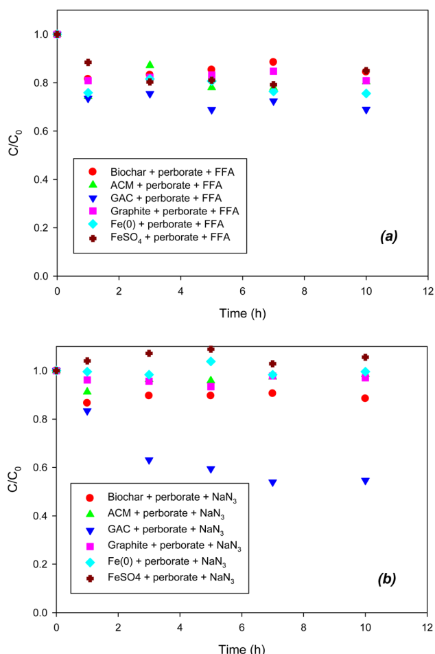
Fig. 4 Effects of (a) FFA ( ^1O_2 scavenger) and (b) NaN_3 ( ^1O_2 and electron transfer scavenger) on the degradation of phenol with perborate in the presence of iron-bearing and carbonaceous materials. The concentration of perborate, the initial concentration of phenol, the amount of iron-bearing and carbonaceous materials, the volume of solution, and initial pH are 250\text{ mg L}^{-1} , 1\text{ mM} , 1\text{ g} (except for GAC: 0.3\text{ g} ), 250\text{ mL} , and \text{pH } 3 , respectively.
