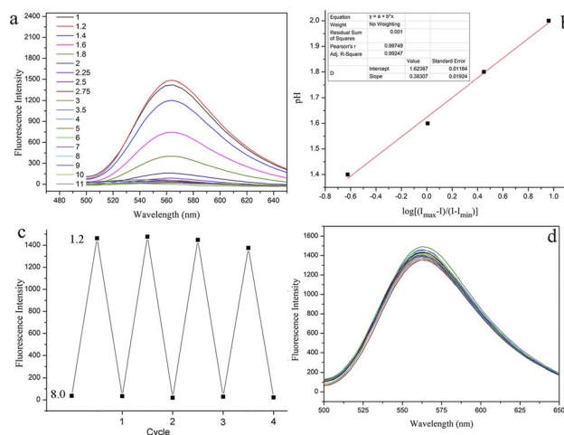
Fig. 6 (a) The fluorescence spectra of CMSM (1 \mu M) under different pH (1.0–11.0). (b) pK_a plot of pH vs. \log((I_{max} - I)/(I - I_{min})) . (c) The reversibility curves of CMSM between pH 8.0 and pH 1.2. (d) The fluorescence spectra of probe CMSM (1 \mu M) in the presence of various anions and cations ( Mg^{2+} , Al^{3+} , Fe^{2+} , Fe^{3+} , Zn^{2+} , Cu^{2+} , Co^{2+} , Ca^{2+} , Ba^{2+} , Ni^{2+} , ClO^- , H_2O_2 , NO_3^- , NO_2^- , F^- , Cl^- , Br^- , I^- , OAc^- , HCO_3^- , SO_4^{2-} , HSO_3^- , S_2O_3^{2-} or S^{2-} , 30 \mu M) at pH 1.2.
