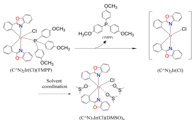
Scheme 5 Inhibition of Lewis donor solvents on catalytic system performance.
