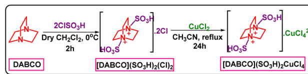
Scheme 1 Preparation of [\text{DABCO}](\text{SO}_3\text{H})_2\text{CuCl}_4 .
