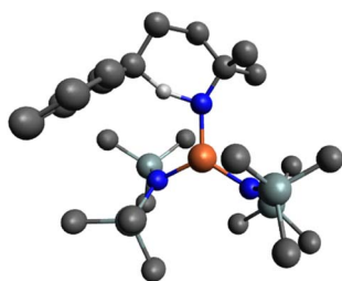
Fig. 9 Ball and stick representation of the optimized transition state TS-i3/i4 by DFT (B3LYP/def2-TZVP) in the pentet spin state. H atoms on all carbons omitted for clarity (Fe orange, N blue, Si mint, C grey, H off-white).
