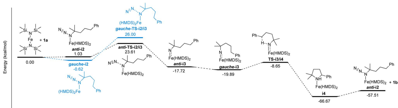
Scheme 1 Reaction coordinate profile of the proposed mechanism for the intramolecular C–H amination catalyzed by Fe(HMDS) 2 . Energies calculated by DFT are given in kcal mol -1 (see Fig. S27–S40† for structures of optimized intermediates and transition states).
