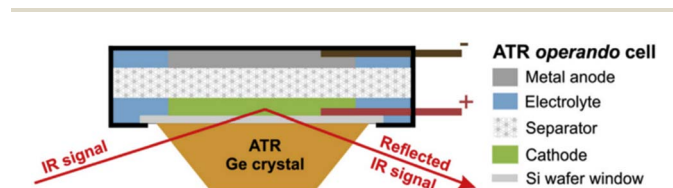
Fig. 8 Schematic representation of the ATR-IR pouch cell on a Ge ATR crystal. Reproduced from ref. 119.
