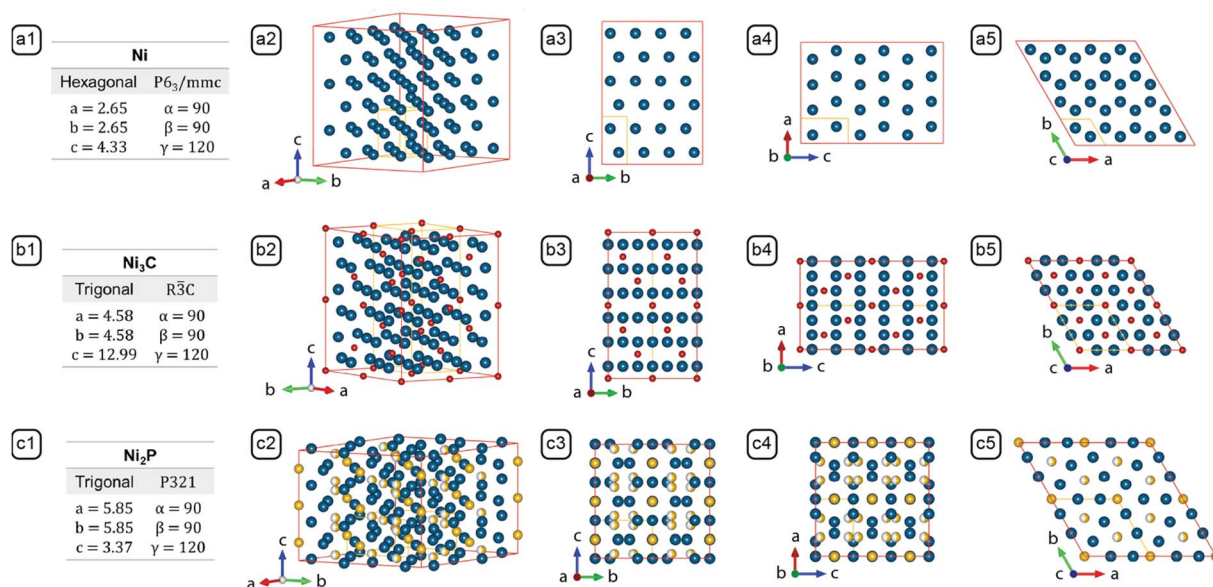
Fig. 4 Lattice parameters and crystal structures of (a) Ni (PDF #45-1027), (b) \text{Ni}_3\text{C} (PDF #06-0697), and (c) \text{Ni}_2\text{P} (PDF #65-9706). Columns: (1) Stoichiometry, crystal system, space group and lattice parameters; (2) crystal model projected along the standard orientation; 31 (3) crystal model projected along [10\bar{1}0] ; (4) crystal model projected along [0110] ; (5) crystal model projected along [0001] . The models outlined by the red edges in columns 2, 3, 4, and 5 consist of multiple unit cells to reveal the resemblance between Ni and \text{Ni}_3\text{C} , and the difference between \text{Ni}_2\text{P} and the former two. The unit cell of each crystal is represented by the yellow lines.
