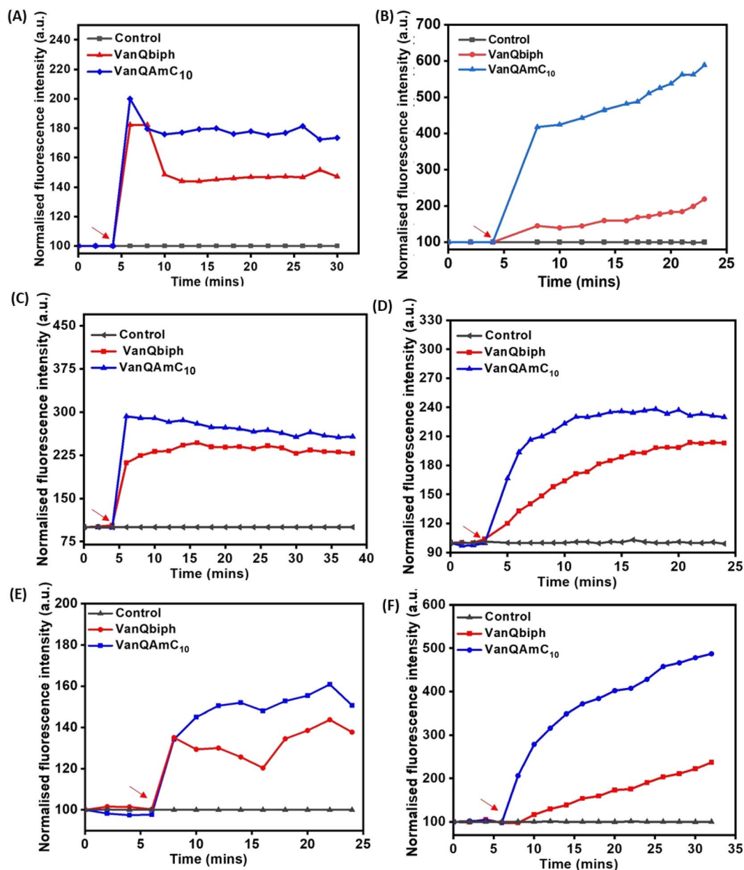
Fig. 2 Membrane-perturbation properties of VanQbiph and VanQAmC 10 . Membrane depolarization against, (A) exponentially growing MRSA, (B) exponentially growing B. subtilis , upon treatment at 10 μM, and (C) stationary phase cells of MRSA upon treatment at 20 μM. Membrane permeabilization against, (D) exponentially growing MRSA, (E) exponentially growing B. subtilis , upon treatment at 10 μM, and (F) stationary phase cells of MRSA upon treatment at 20 μM. Red arrows indicate compound addition. The error percentage between replicates of an experiment was lesser than 5%. The images are representative of results from three independent experiments.
