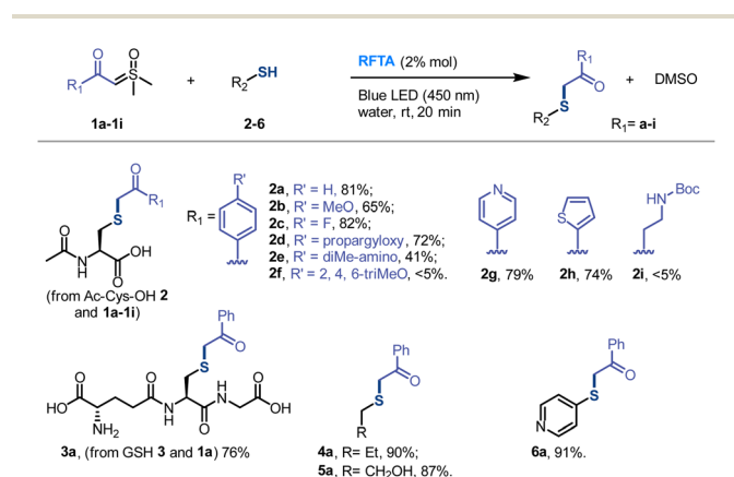
Fig. 2 Scope of the S–H insertion of sulfoxonium ylides. Conditions: 1 (1 mmol, 2 equiv.), thiol 2–6 (0.5 mmol, 1 equiv.) and RFTA (2% mol) under light irradiation (450 nm) for 20 min in water (8 mL) at rt. Isolated yields were reported.
