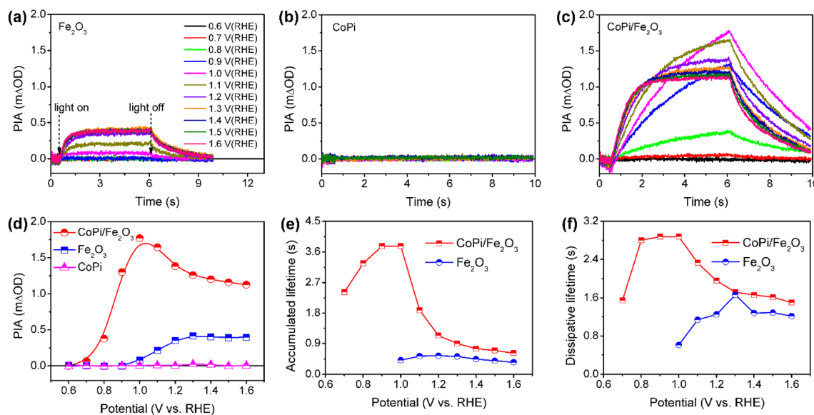
Fig. 3 PIA responses at various potentials for bare \text{Fe}_2\text{O}_3 (a), CoPi (b) and CoPi/ \text{Fe}_2\text{O}_3 (c). (d) PIA amplitudes following increasing potential extracted from Fig. 2a–2c. Average lifetimes ( \tau_{\text{ave}} ) of (e) accumulated and (f) dissipative processes for bare \text{Fe}_2\text{O}_3 and CoPi/ \text{Fe}_2\text{O}_3 photoanodes in (a and c). Pump wavelength is 456 nm ( 5 \text{ mW cm}^{-2} ); probe wavelength is 694.3 nm; colors of curves at different potentials in (a–c) are identical.
