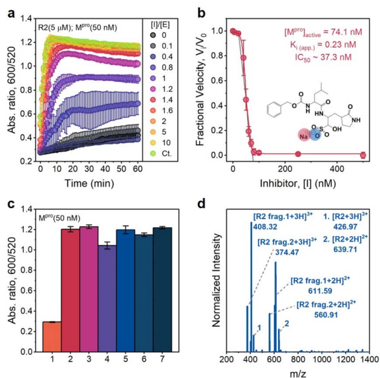
Fig. 5 Inhibition and selectivity assays. (a) Time progression of the ratiometric signal (Abs 600 /Abs 520 ) in inhibitor assays. An increasing molar ratio of [inhibitor]/[M Pro ] from 0 to 10 was employed. The control curve (Ct.) designates an inhibitor only without an M Pro additive. Error bar = standard deviation of the three samples. (b) A typical inhibition titration curve fitted with the Morrison equation (eqn. (2)) is shown for the competitive inhibitor, GC376. The inset shows the chemical structure of the GC376 inhibitor. Error bar = relative standard deviation of the three samples. (c) Sensor activation by mammalian proteins (50 nM). 1 = positive control only with M Pro , 2 = trypsin, 3 = thrombin, 4 = hemoglobin, 5 = BSA, 6 = α-amylase (50 U per mL), and 7 = negative control without M Pro . Error bar = standard deviation of the three samples. (d) ESI-MS data confirm the cleavage of the R2 peptide by trypsin.
