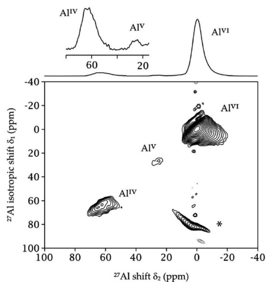
Fig. 9 Experimental DNP-enhanced 1 H– 27 Al CP MQMAS NMR spectrum of \gamma -alumina nano-powder impregnated with 16 mM PyrroTriPol-OMe in TCE, recorded at 18.8 T, 40 kHz MAS frequency and ~110 K, giving a DNP enhancement factor \epsilon_{\text{on/off}} \sim 90 . Spinning sidebands are indicated with a star.
