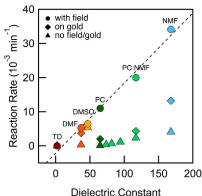
Fig. 3 Rate of consumption of 1 in TD (dark red), DMF (orange), DMSO (yellow), PC (dark green), NMF (blue), and mixtures of PC and NMF (light green) in ratios of 1 : 10, 2 : 10, 4 : 10, 1 : 1 (from left to right) plotted against solvent dielectric. Data for rates are measured from STM-BJ measurements using an applied bias of 100 mV (circles), exposure to gold (diamonds) and without an applied field or exposure to gold (triangles). The dashed line is a linear fit to the data.
