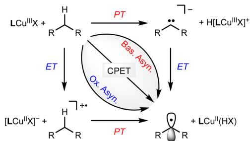
Scheme 2 Possible mechanisms of PCET by LCu III FG complexes.
