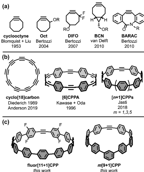
Fig. 1 (a) Examples of strained alkynes developed for copper-free click chemistry. (b) Strained alkynes in the field of carbon nanomaterials. (c) New strained alkyne-containing [n+1] CPPs described in this work.
