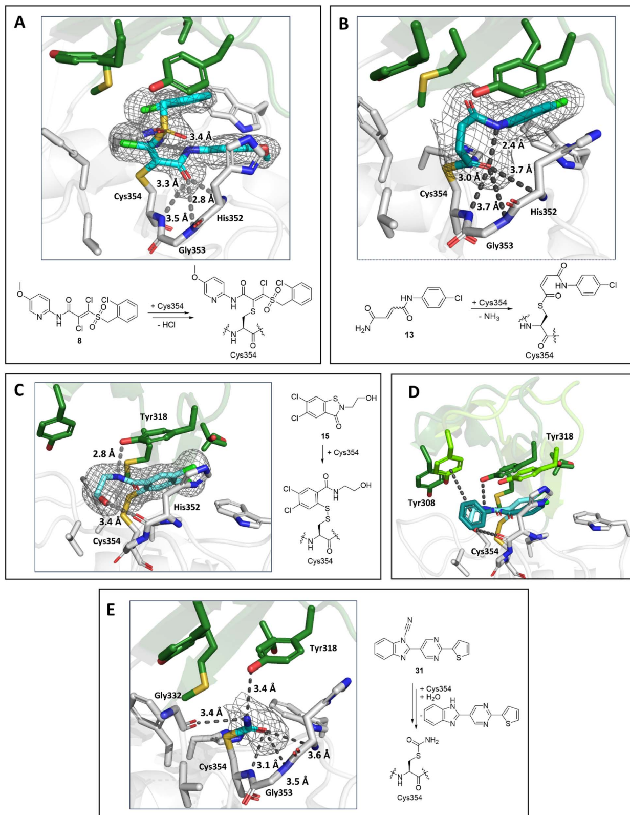
Fig. 9 Views from crystal structures of the complex derived by reaction of \text{Ldt}_{\text{Mt2}} with inhibitors 8 , 13 , 15 and 31 . (A) Active site view of \text{Ldt}_{\text{Mt2}} reacted with 8 (cyan, PDB 8A1O). (B) Active site view of \text{Ldt}_{\text{Mt2}} reacted with 13 (teal, PDB 8A1N). (C) Active site view of \text{Ldt}_{\text{Mt2}} reacted with 15 (cyan; PDB 8A1K). (D) Superimposition view from crystal structures of \text{Ldt}_{\text{Mt2}} in complex with 15 ( \text{Ldt}_{\text{Mt2}} -bound 15 in cyan, active site "lid" in dark green; PDB 8A1K) and in complex with ebisen ( \text{Ldt}_{\text{Mt2}} -bound ebisen in teal, active site "lid" in light green; PDB 6RRM). 19 (E) Active site view of \text{Ldt}_{\text{Mt2}} reacted with 31 (cyan; PDB 8AHO). Active site views in (A–E) are shown as observed in chain A. mF_o - DF_c polder OMIT maps 59 contoured at 3.0\sigma , carved around Cys354 bound 8 , 13 , 15 and 31 are shown in grey mesh. Polar interactions are shown in grey dashes. The crystallographically assigned products are consistent with those observed by mass spectrometry (Fig. S10 and S13†).
