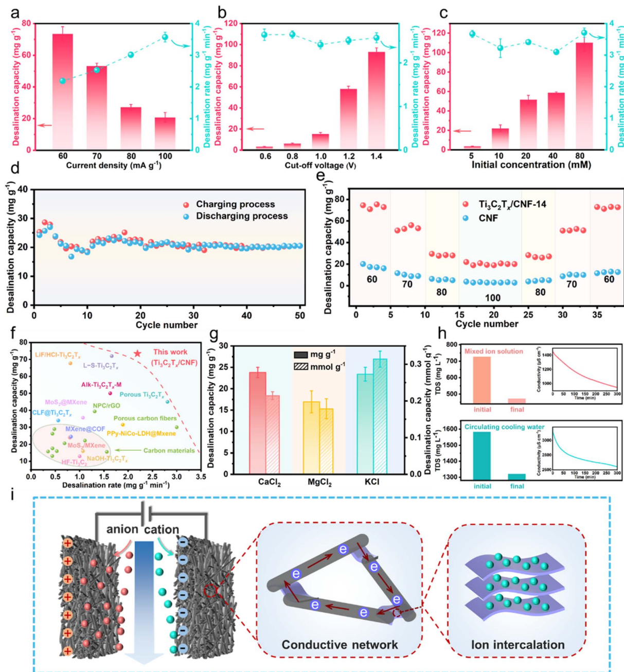
Fig. 6 Capacity and rate of desalination of \text{Ti}_3\text{C}_2\text{T}_x/\text{CNF} -14 at different current densities (a), cutoff voltages (b), and \text{NaCl} initial concentration (c). (d) Cycling and regeneration performance of \text{Ti}_3\text{C}_2\text{T}_x/\text{CNF} -14 at 100 \text{ mA g}^{-1} over 50 cycles. (e) Desalination capacity of \text{CNF} and \text{Ti}_3\text{C}_2\text{T}_x/\text{CNF} -14 at different current densities. (f) Comparison of the desalination performance of \text{Ti}_3\text{C}_2\text{T}_x/\text{CNF} -14 with other carbon- and MXene-based electrode materials. (g) Mass and molar desalination capacity of \text{Ti}_3\text{C}_2\text{T}_x/\text{CNF} -14 for \text{CaCl}_2 , \text{MgCl}_2 , and \text{KCl} . (h) TDS-removal capacity of \text{Ti}_3\text{C}_2\text{T}_x/\text{CNF} -14 for a mixed ion solution (up) and circulating cooling water (down). Inset shows the change in conductivity. (i) \text{Ti}_3\text{C}_2\text{T}_x/\text{CNF} -14 capacitive deionization (schematic).
