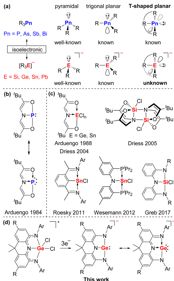
Fig. 1 (a) Molecular shapes oftricoordinate heavier group 14/15 compounds. (b) The first isolable T-shaped planar phosphorus compound. (c) Geometrically constrained group 14 precursors. (d) Present work.
